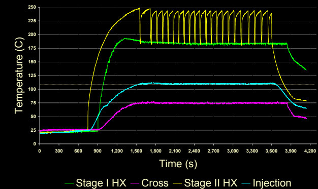
Time After Engine Start vs. Temperature
